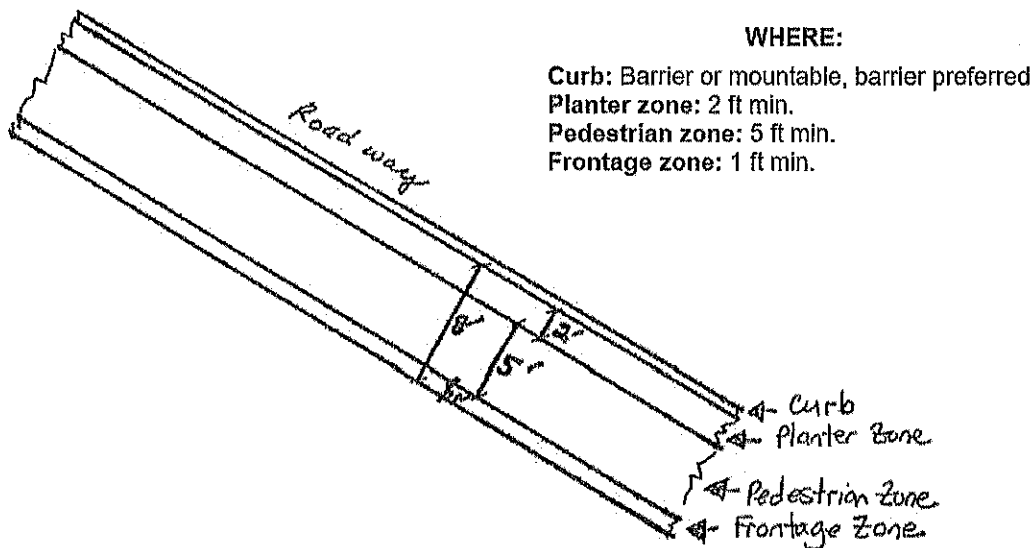
Figure 10.2.5-1. Pre-Approved Design for Sidewalk with Planter Zone.
